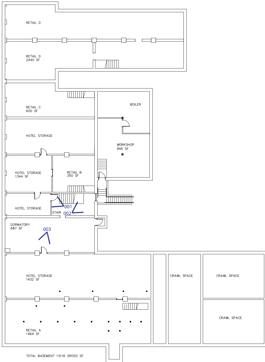
BASEMENT FLOOR PLAN N.T.S.
